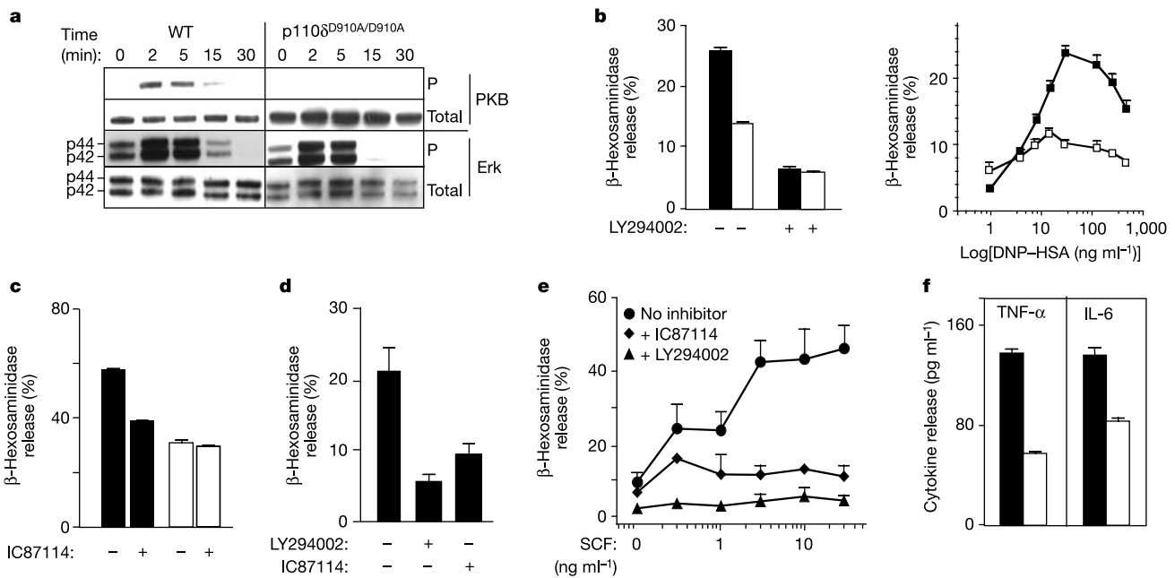
Figure 3 Effect of p110δ inactivation on FcεRI-induced BMMC responses. a–c , Signalling ( a ) and β-hexosaminidase release ( b , c ) in BMMCs stimulated with IgE–antigen. Right panel of b : dose titration of DNP–HSA. d , Effect of inhibitors on degranulation of human mast cells challenged with antigen (1 ng ml -1 ). e , Effect of PI(3)K inhibitors on SCF-potentiated human mast cell degranulation (using a suboptimal antigen
