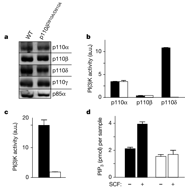
Figure 1 Effect of p110δ inactivation on PI(3)K expression and activity. a , Expression of class I PI(3)K isoforms in total cell lysates (50 μg per lane), assessed by immunoblotting. WT, wild type. b , In vitro lipid kinase activity of class IA PI(3)Ks. p110 isoforms were immunoprecipitated using isoform-specific antibodies, and tested for associated lipid kinase activity (presented as arbitrary units (a.u.)). c , In vitro lipid kinase activity of BMMC class IA PI(3)Ks, isolated using Y p VPMLG (where Y p is phosphotyrosine) peptide complexes. d , In vivo PIP 3 levels in BMMCs stimulated with or without 100 ng ml -1 SCF for 10 min. Filled bars, wild type; open bars, p110δ D910A/D910A .
